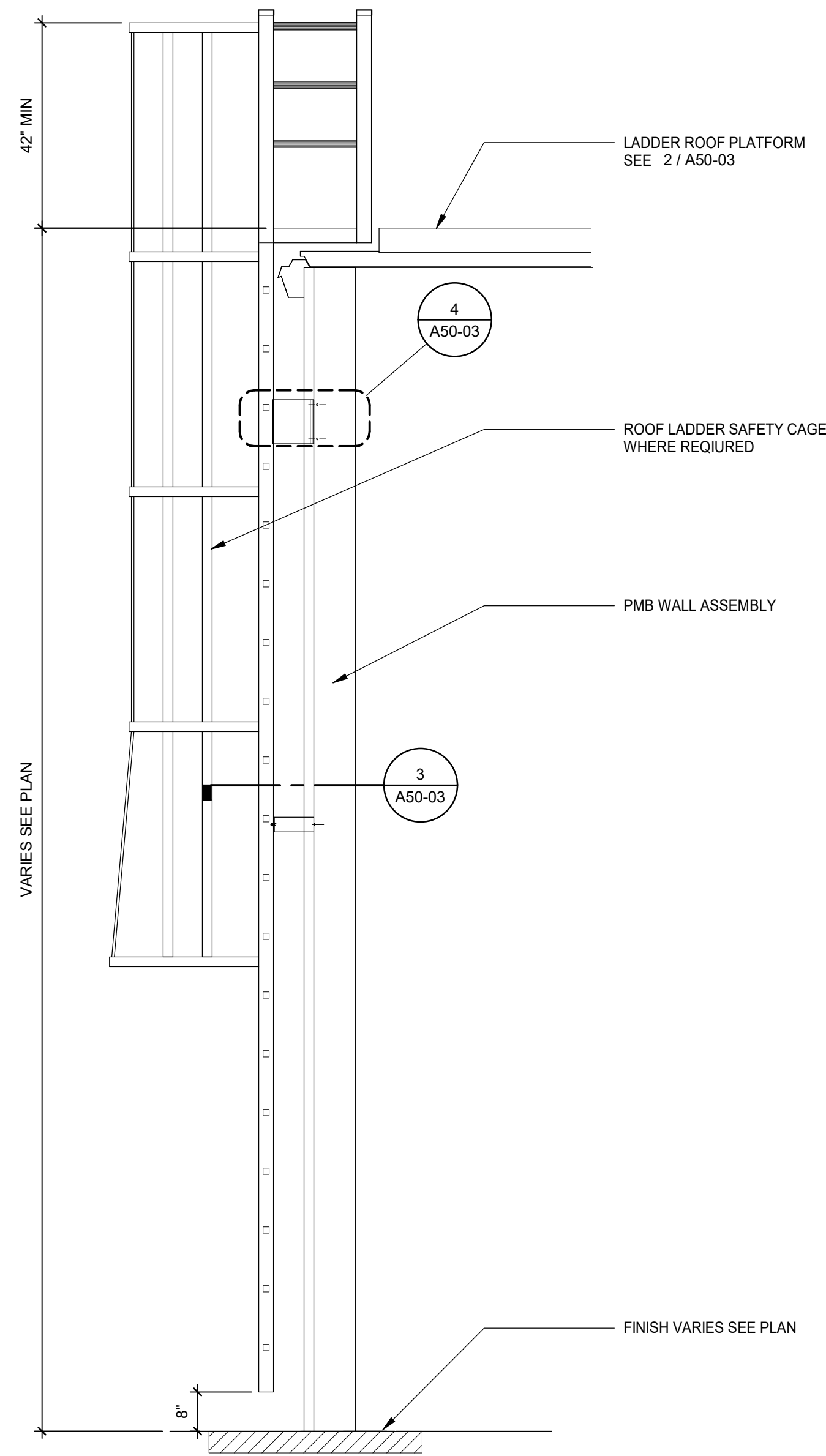
1 A50-03 LADDER SIDE ELEVATION SCALE: 1/2" = 1'-0"
