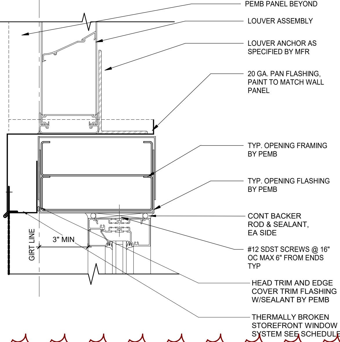
13 LOUVER SILL -WINDOW HEAD SCALE: 3" = 1'-0"
