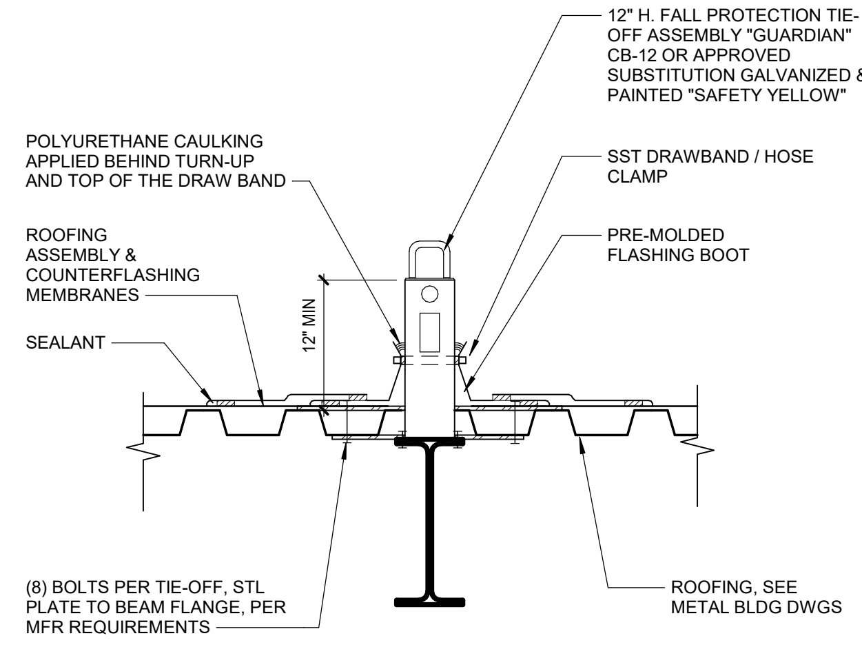
5 A50-03 FALL PROTECTION TIE OFF ASSEMBLY SCALE: 1 1/2" = 1'-0"
