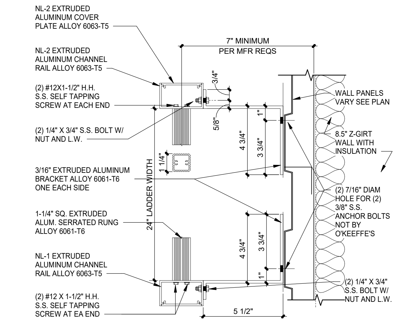
3 A50-03 LADDER BRACKET PLAN VIEW SCALE: 3" = 1'-0"
