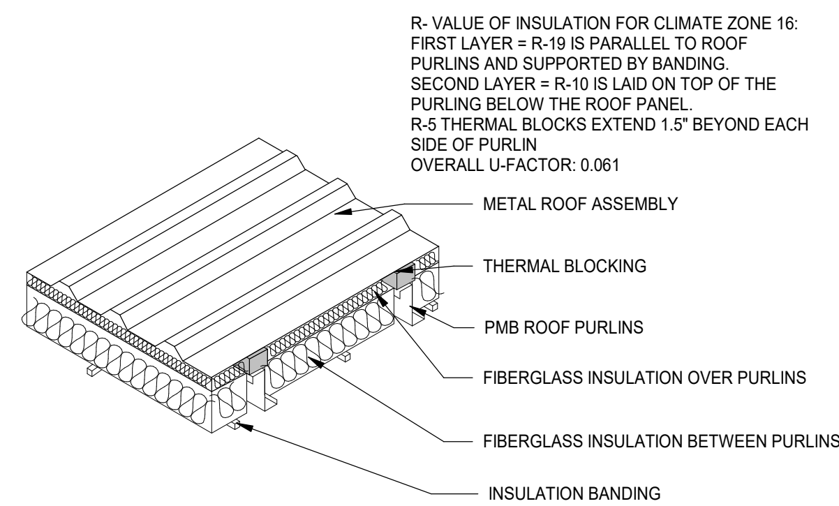
6 A50-03 ROOF PRESCRIPTIVE ENVELOP REQUIREMENTS SCALE: 1/2" = 1'-0"
