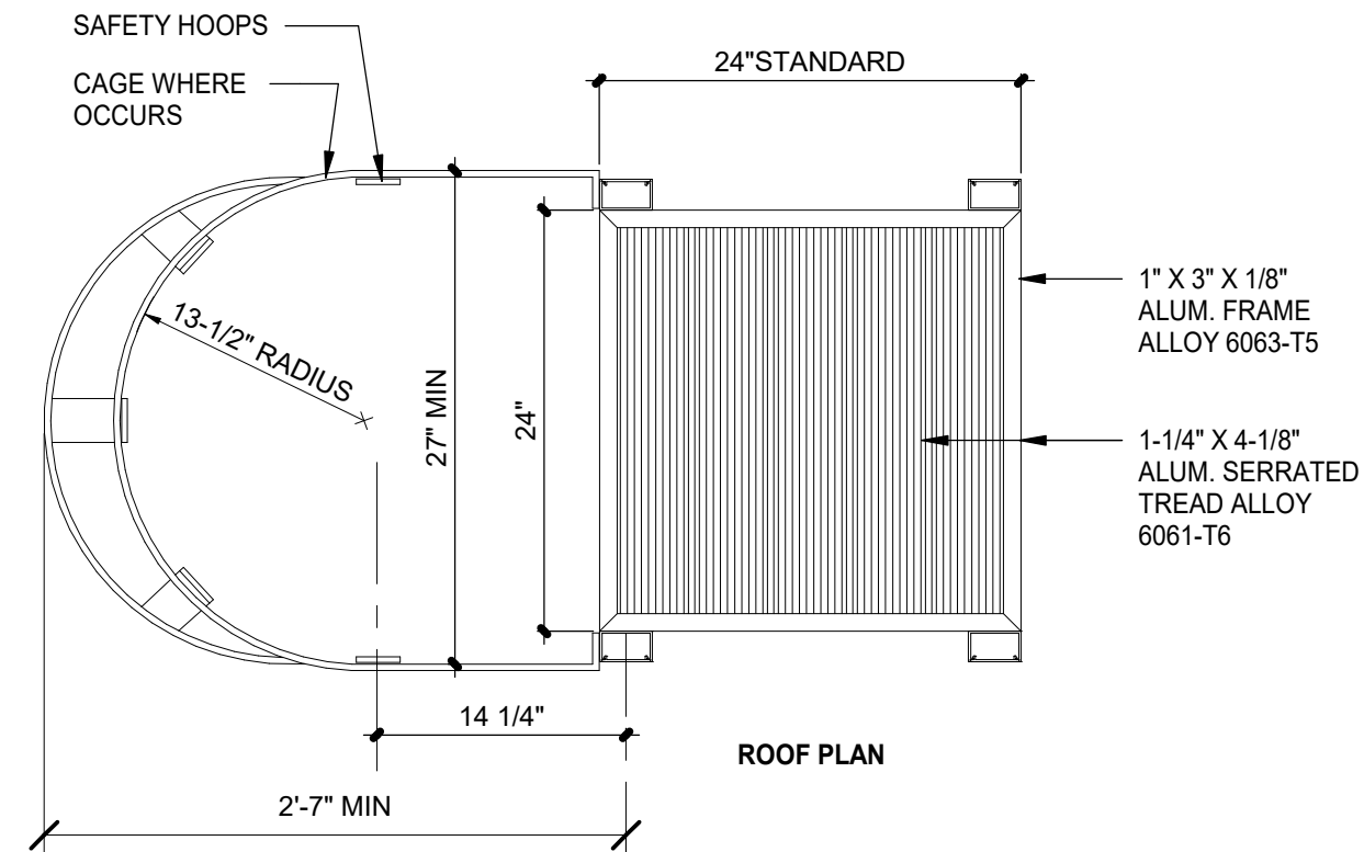
2 A50-03 LADDER ROOF PLATFORM SCALE: 1" = 1'-0"
