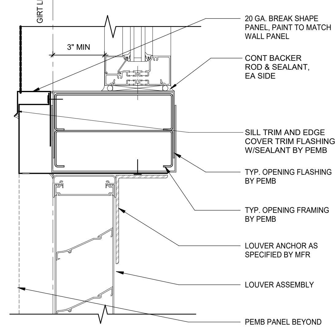
11 LOUVER HEAD -WINDOW SILL SCALE: 3" = 1'-0"
