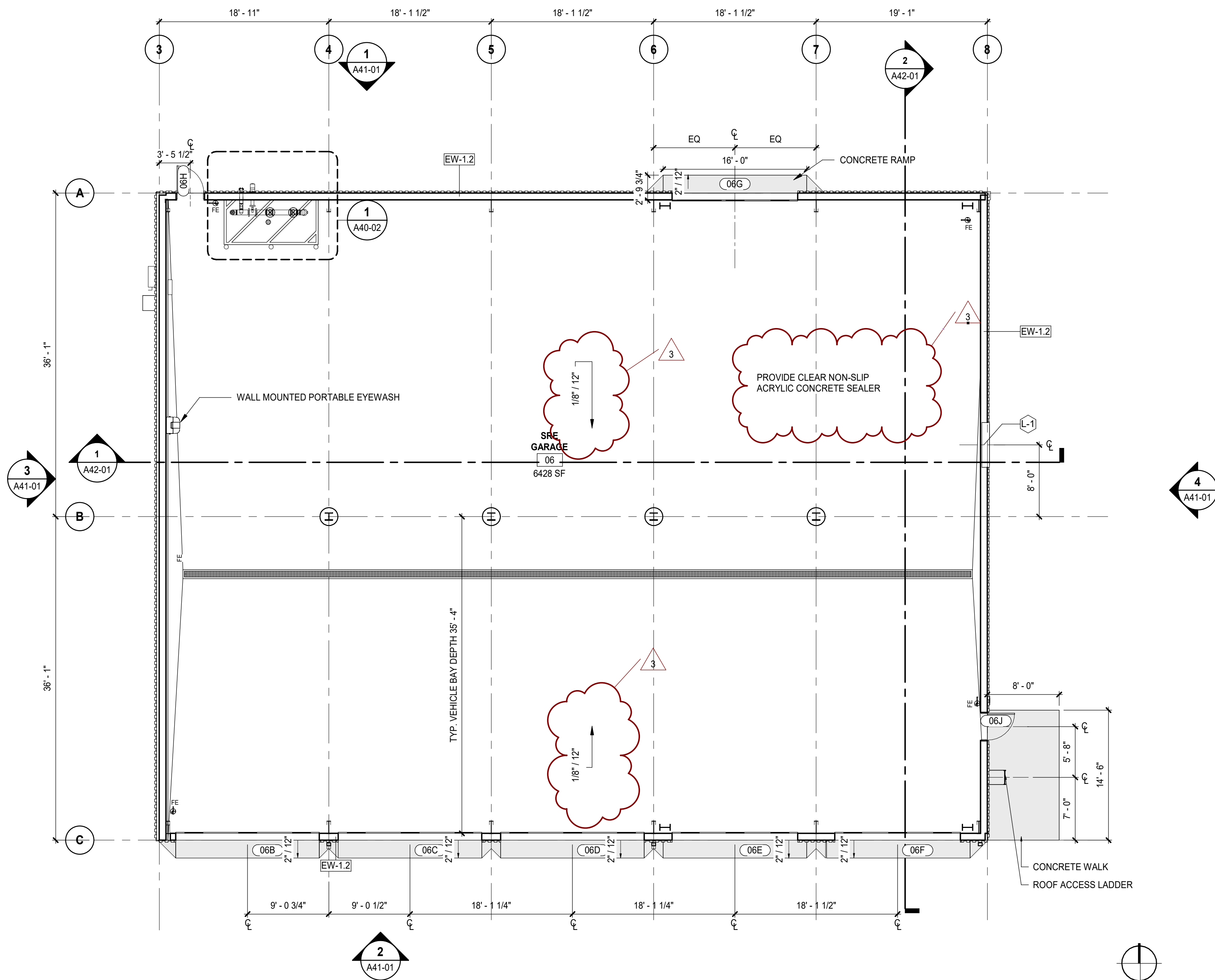
1 LEVEL 1 OVERALL FLOOR PLAN SCALE: 1/8" = 1'-0"
