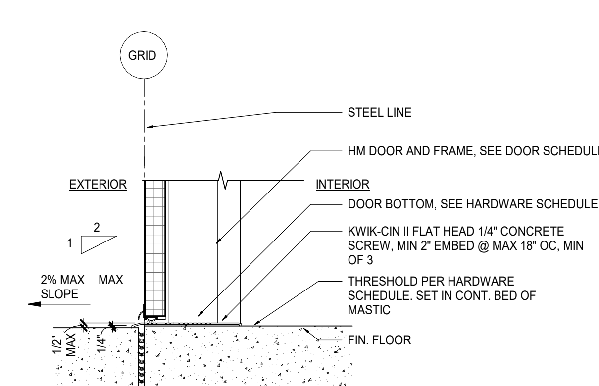
3 EXTERIOR DOOR THRESHOLD SCALE: 1 1/2" = 1'-0"
