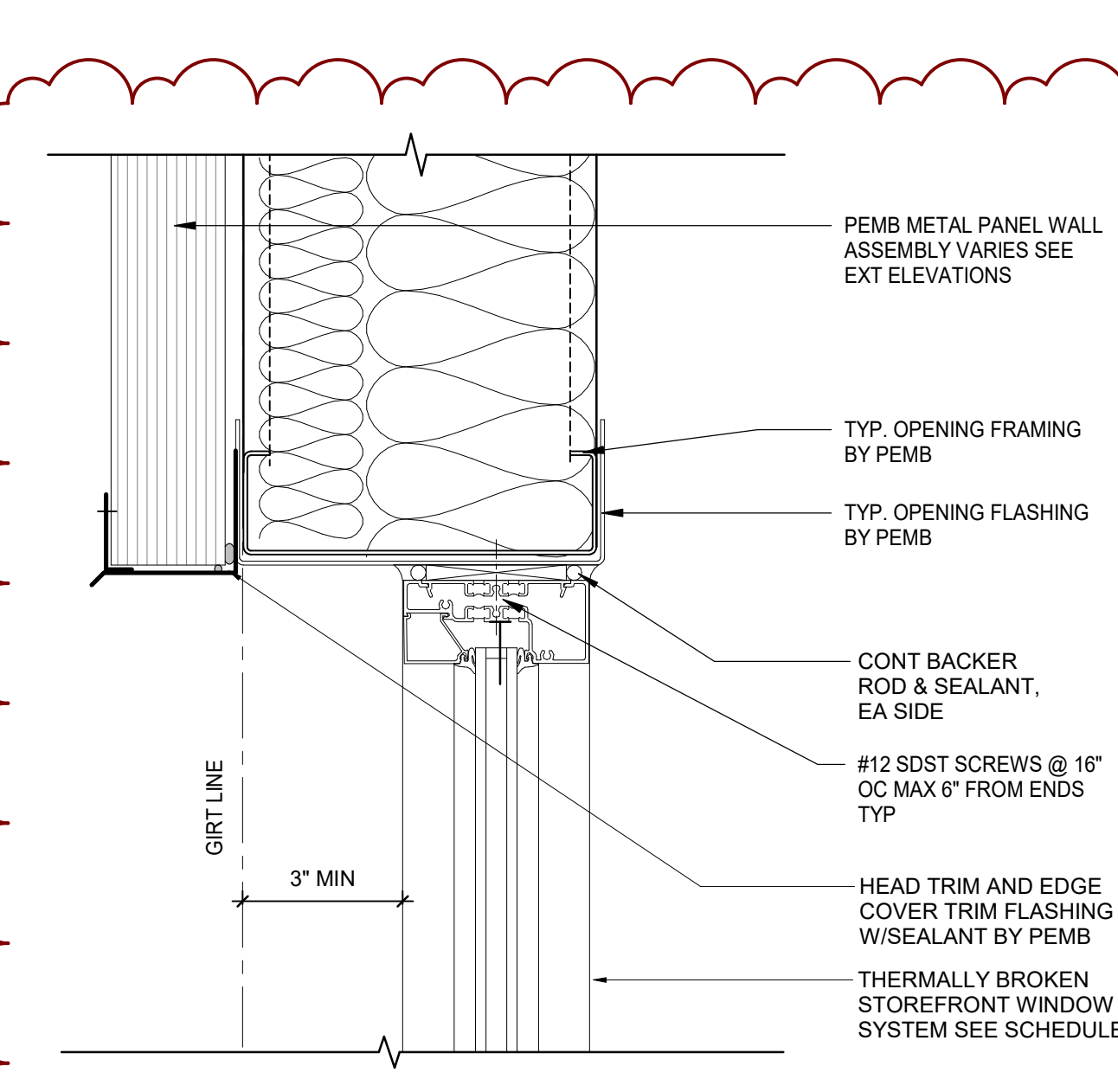
6 WINDOW HEAD SCALE: 1 1/2" = 1'-0"
