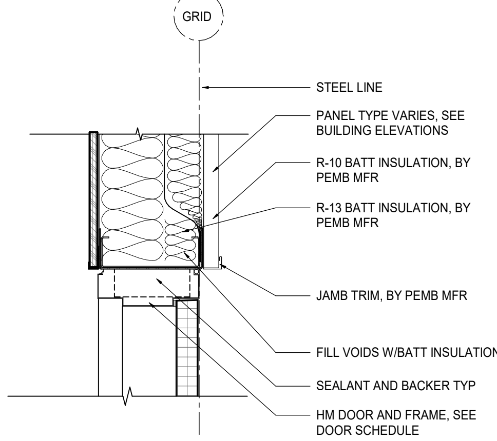
2 EXTERIOR DOOR JAMB SCALE: 1 1/2" = 1'-0"
