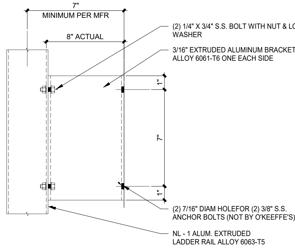
4 A50-03 LADDER BRACKET SIDE VIEW SCALE: 3" = 1'-0"
