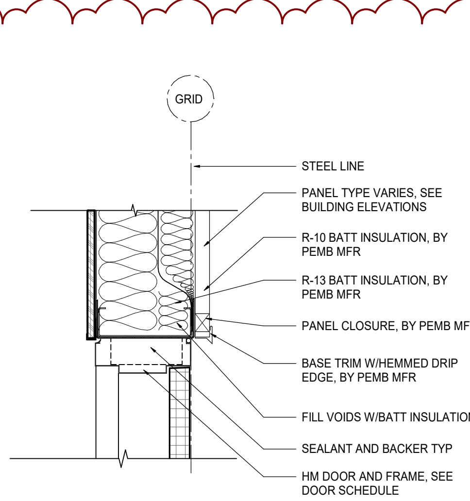
1 EXTERIOR DOOR HEAD SCALE: 1 1/2" = 1'-0"
